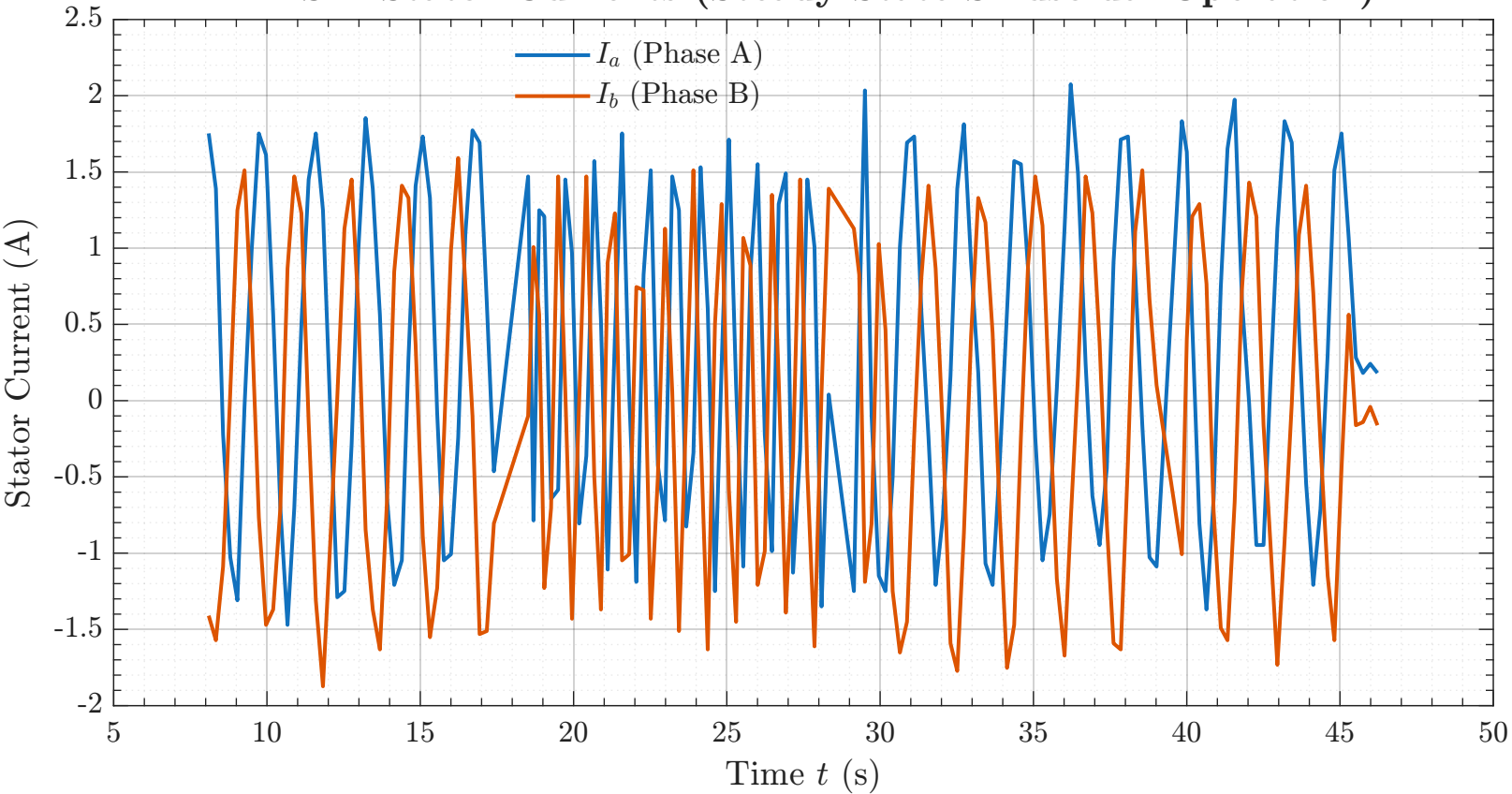
PMSM Stator Currents (Steady-State Sinusoidal Operation)
